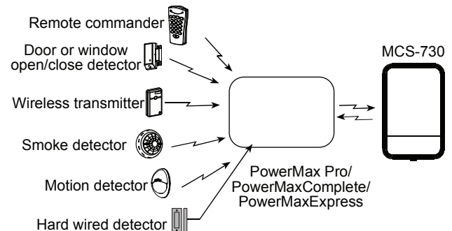
Figure 2- Typical Integration with the Alarm System
